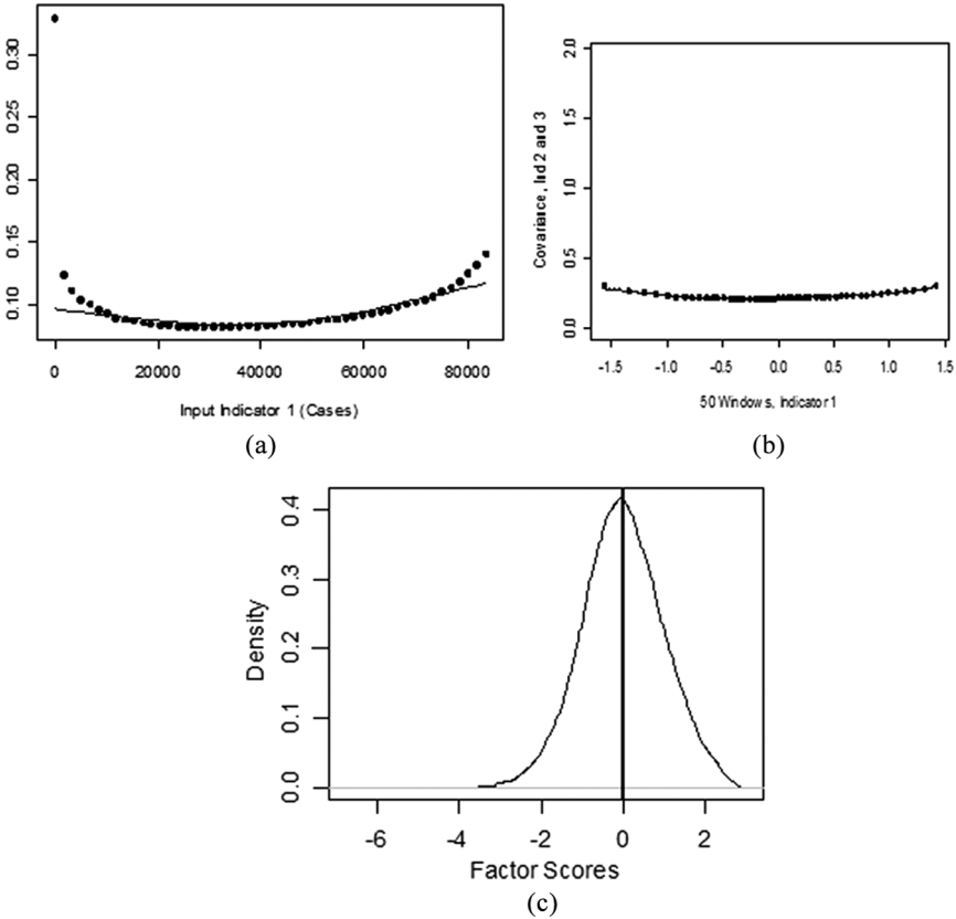
FIGURE 1 (a) All 42 MAMBAC curves demonstrated this U-shaped pattern. (b) All 105 MAXCOV curves demonstrated this flattened pattern. (c) The single L-mode curve was unimodal. Every one of these patterns is indicative of dimensional structure.
